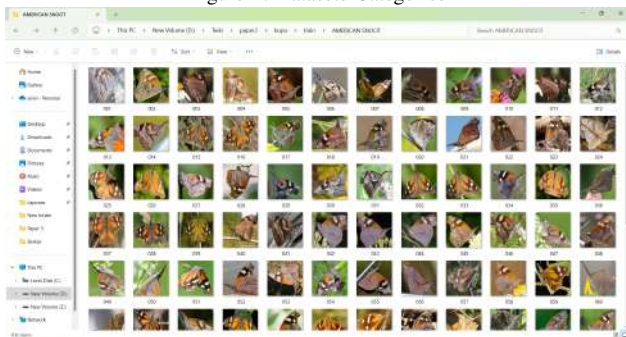
Figure 5. Image Datasets
