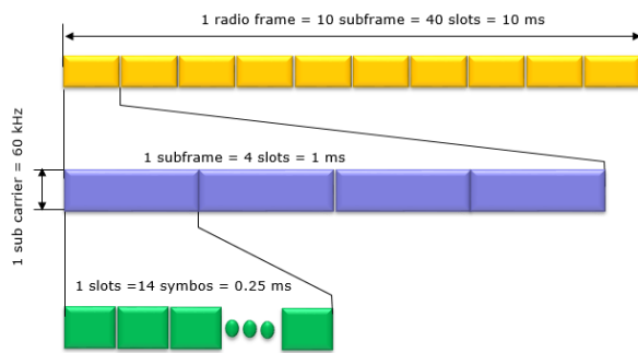
Figure 5. 5G Frame Format
