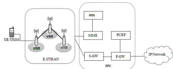
Figure 2. LTE Network Architecture
