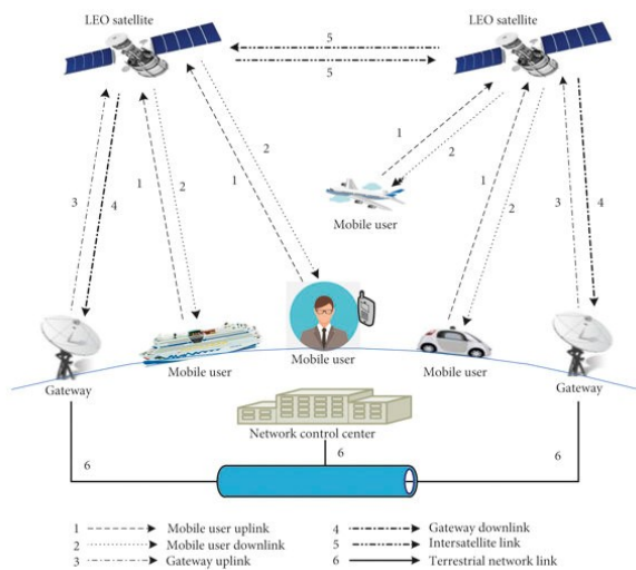
Figure 1. LEO Satellite system
