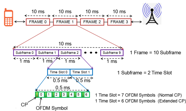
Figure 3. LTE Frame Format
