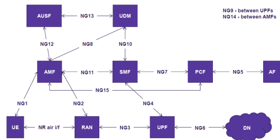
Figure 4. 5G Network Architecture
