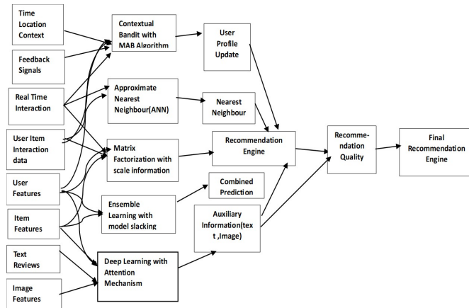
Figure 1. Model Architecture of the Proposed Recommendation Process
